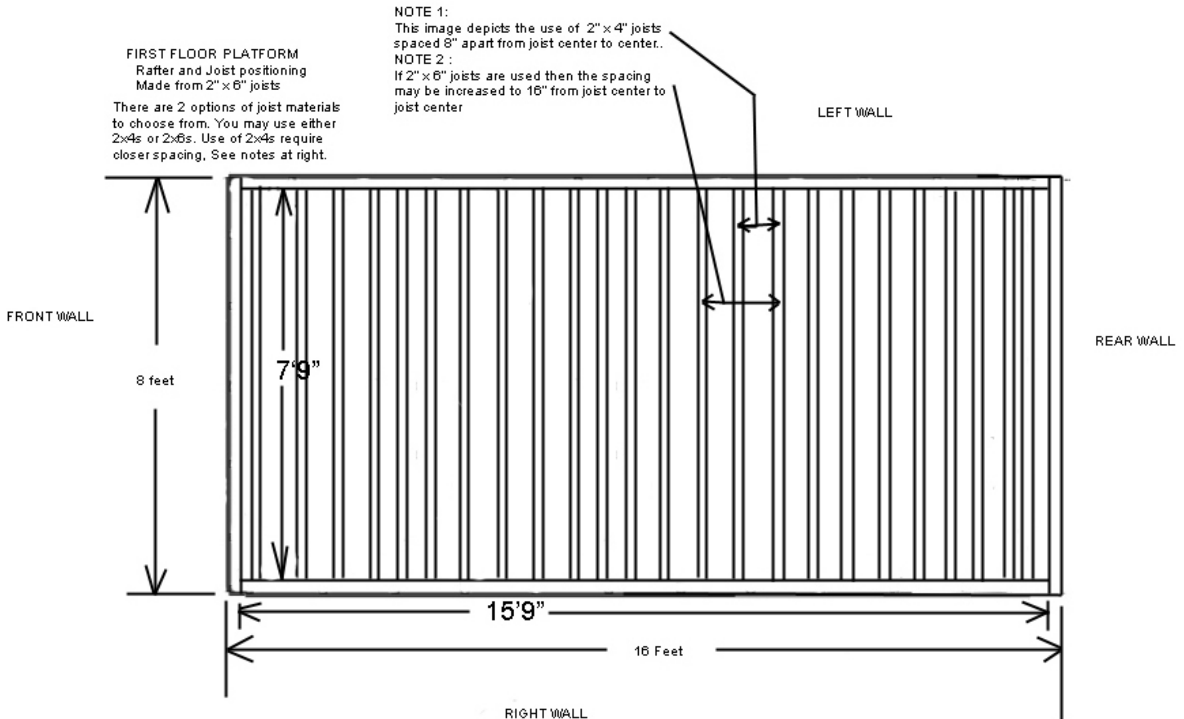
8'x16' Flat Roof Tiny House (First Floor - floor joist platform) Showing the layout, and location of floor joists for 1st floor
